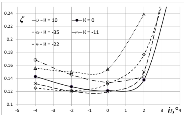
Figure 5 – The experimental data for channel diffuser
