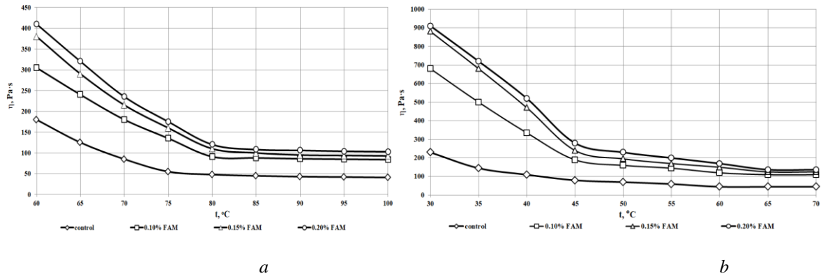
Fig. 6. Dependence of the viscosity of gelling systems “gelling agent + FAM” on the temperature: a – in the agar-based samples; b – in the pectin-based samples
