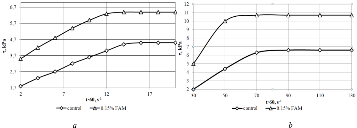
Fig. 7. Dependence of the critical shear stress of gel systems “gelling agent + FAM” on the duration of maturation: a – on agar; b – on pectin
