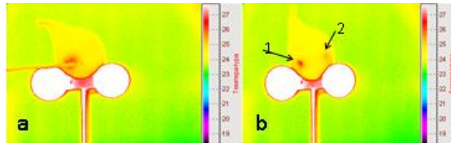
Fig. 2. Thermograms of pears with signs of damage
