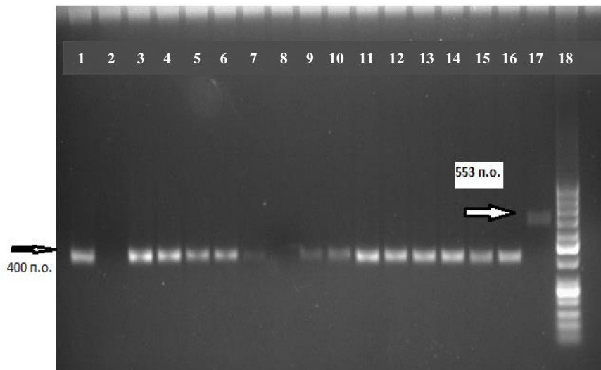
Fig. 6 – Electrophoregram of PCR products with a pair of specific oligonucleotide primers for the groEL gene:
