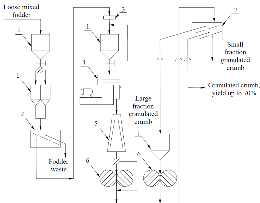
Figure 3. Scheme of the technology of granulation of mixed fodders with getting granulated crumb
