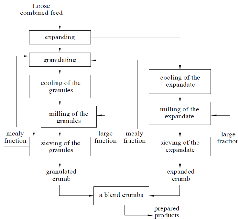
Figure 5. Scheme of the granulation technology with using pre-expanding and obtaining granulated crumb and expanded crumb
