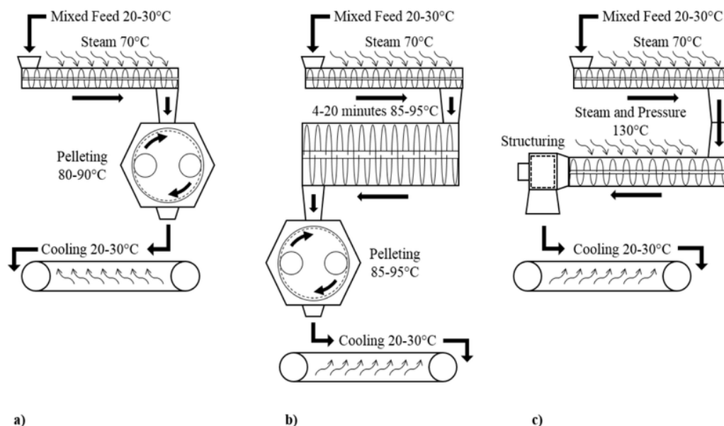
Figure 4. Scheme of the granulation of compound feed using of preliminary wet-heat treatment.
