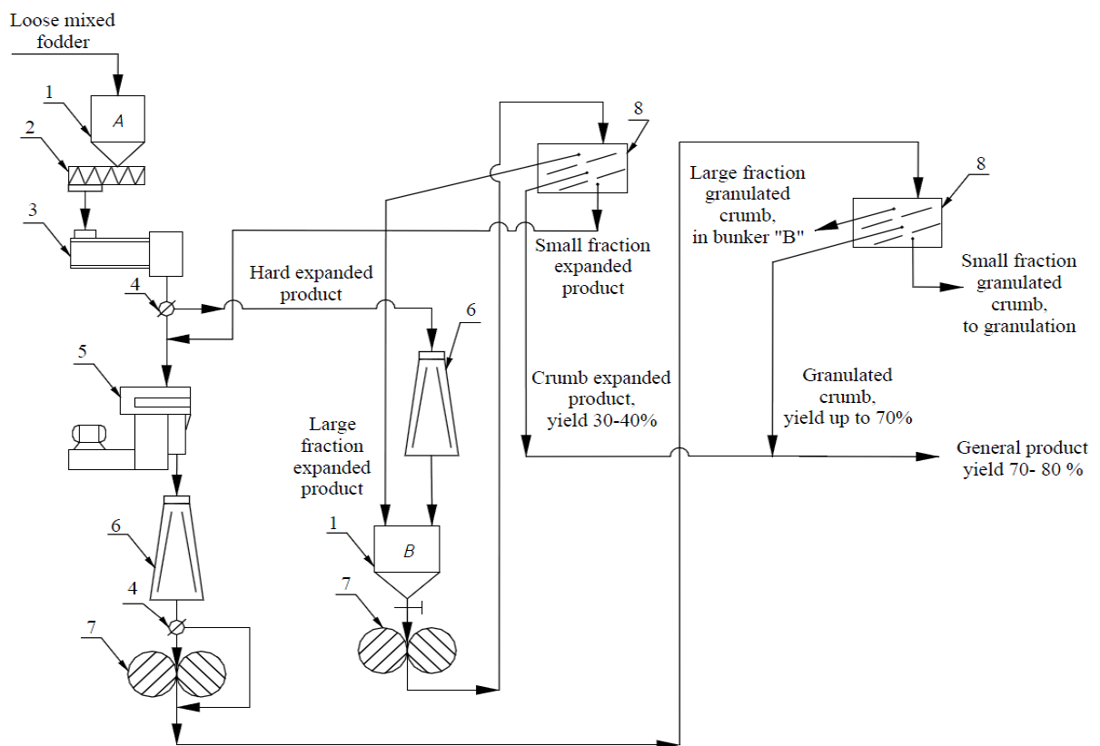
Figure 6. Improvement scheme of the granulation technology with obtaining granulated crumb and expanded crumb: 1 – temporary storage bunker; 2 – moisturizer; 3- expander; 4 – changeover valve; 5 – granulator; 6 – cooler; 7 – crusher; 8 – separator, sifting machine.
