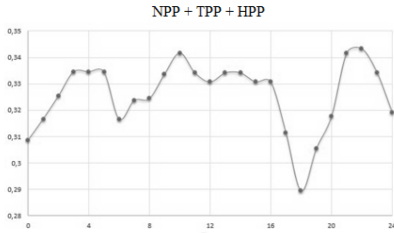
Fig. 10 – Change of performance efficiency criterion for the first option of joint operation of three power plants during the day
