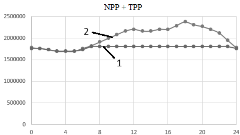
Fig. 5 – Curves of changes in electric power yield for the second option of two power units (1) and system demand (2) per day
