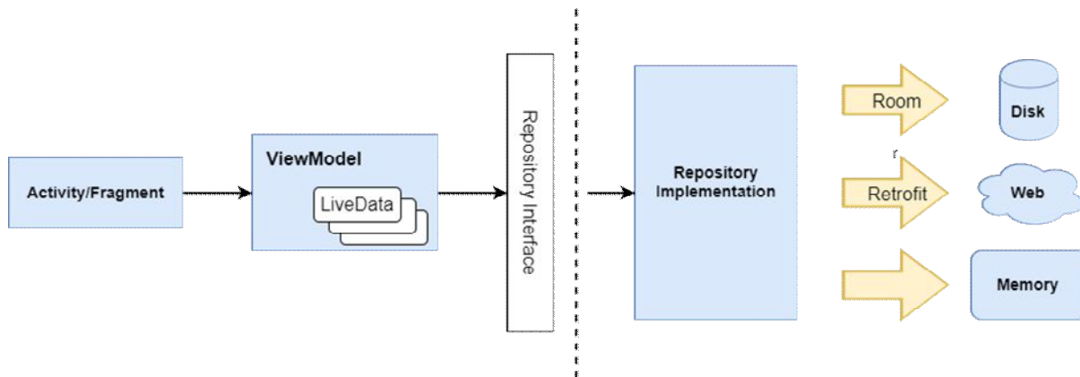
Fig. 4 – "Clean architecture" scheme ft. Google
