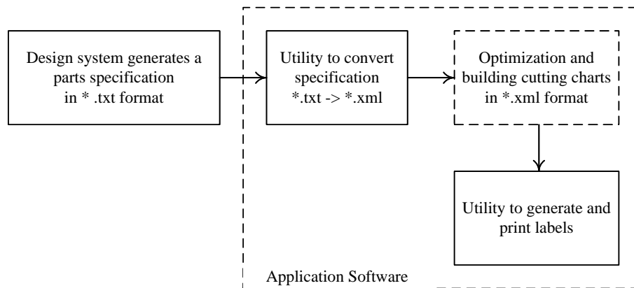
Fig. 1. The information processing diagram in the profile cutting process.
